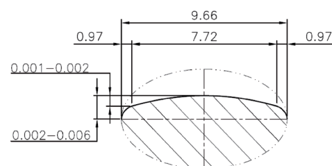
DETAIL A-LOGARITHMIC PROFILE AT TRACK
